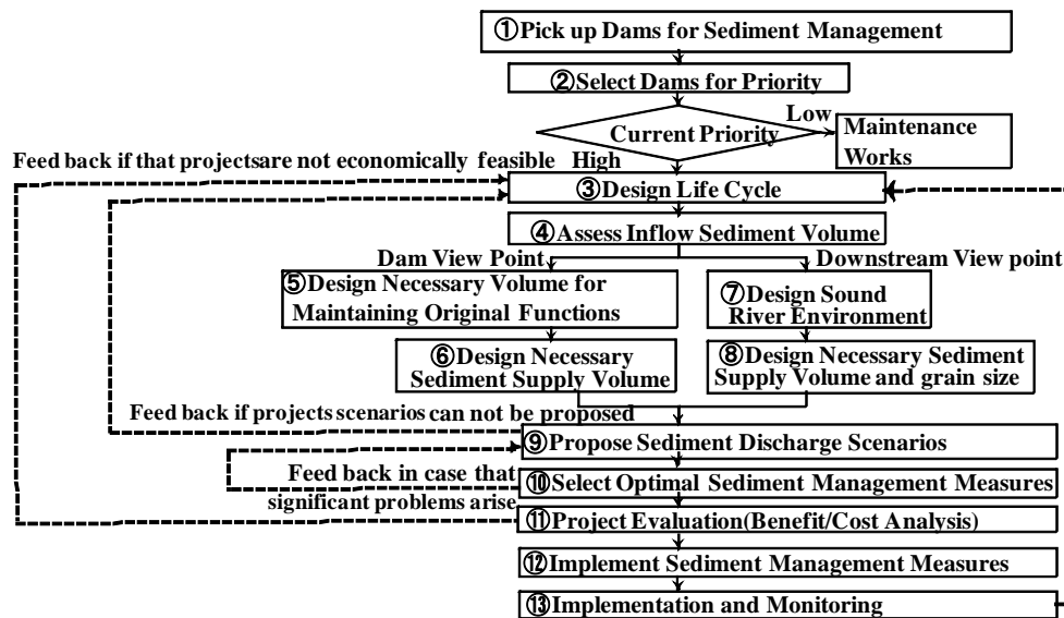
Figure 10. Flowchart for setting up sediment management strategy
