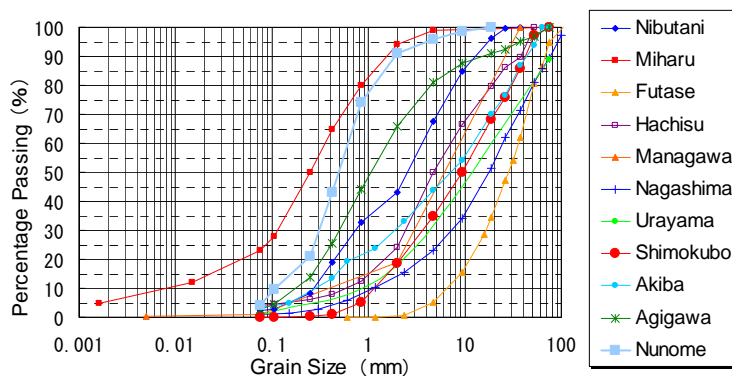
Figure 6. Grain size distributions of sediment replenishment
