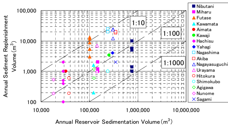
Figure 5. Relationship between annual reservoir sedimentation and replenishment volumes in Japan.
