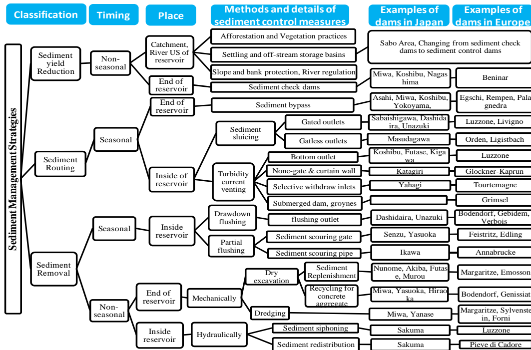
Figure 4. Classification of strategies of sediment control in Japanese and European reservoirs.
