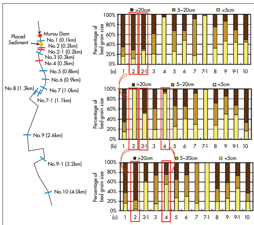
Figure 10: Variations of river bed material size in 13 cross sections along Uda River
