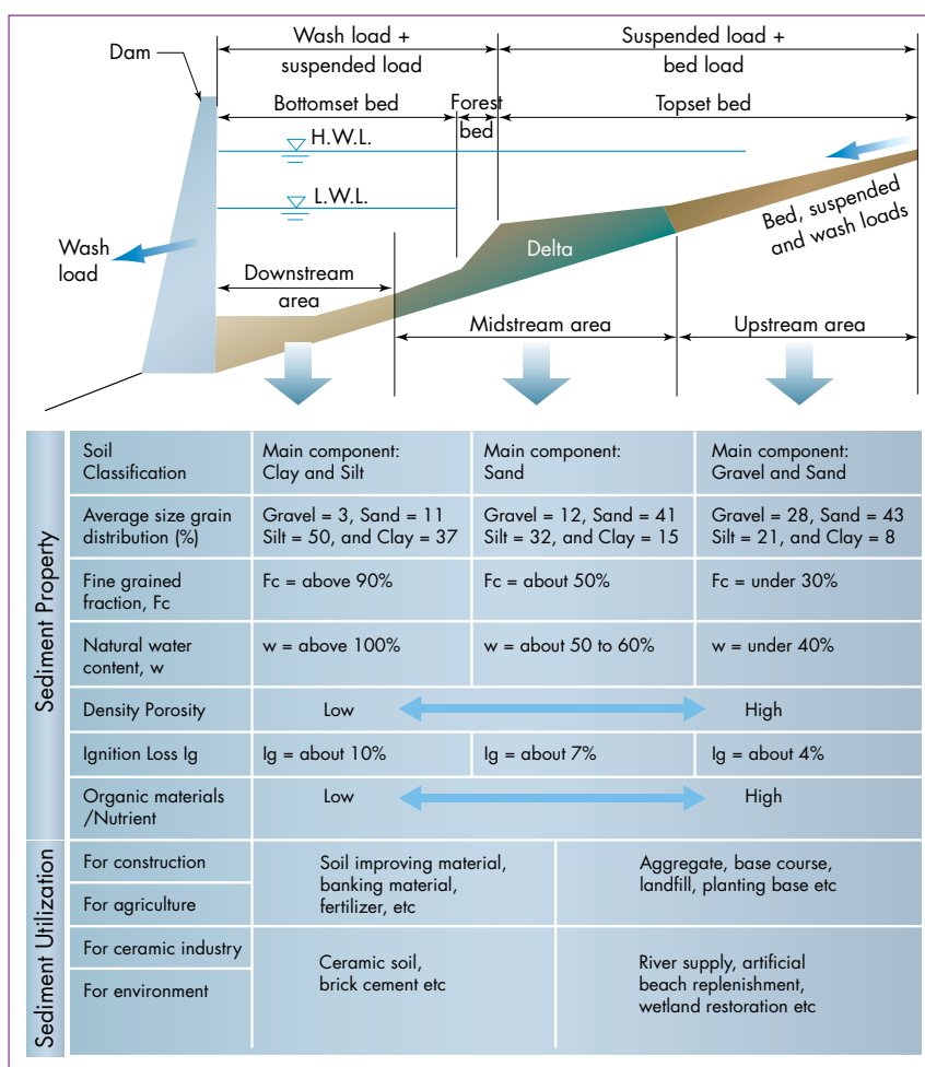
Figure 1: Delta formation and properties of deposited sediments within reservoirs and applications of different types of sediments
