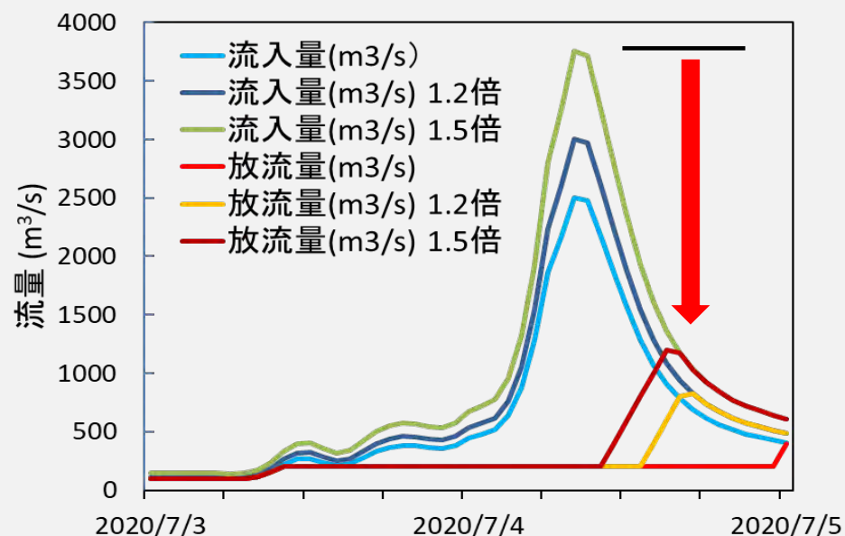
200m 3 /s一定放流
