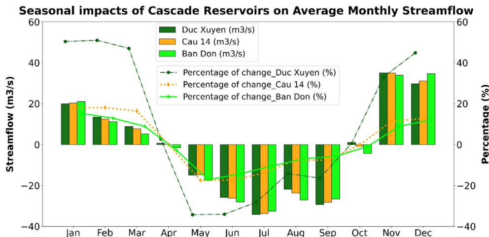
FIGURE 9 Seasonal differences by months between regulated and natural streamflow at three stations in the USBR. Bars (left y-axis) show the difference in magnitude (m 3 /s) whereas lines (right y-axis) show the difference in percentage values.
