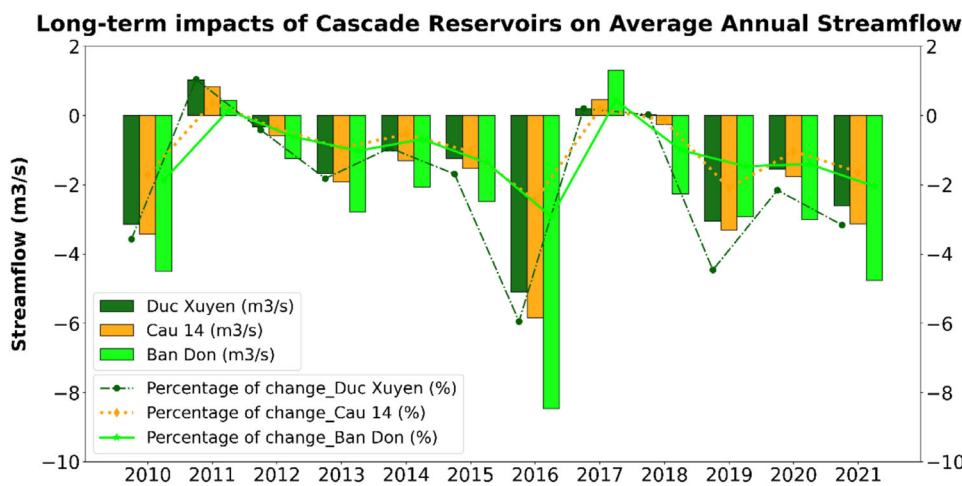
FIGURE 8 Long-term difference in average annual streamflow values between regulated and natural streamflow. Bars (left y-axis) show the difference in magnitude (m 3 /s) whereas lines (right y-axis) show the difference in percentage values.
